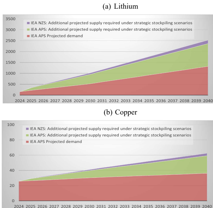
Fig. 5 | Projected supply requirements for copper under IEA APS and NZS, including global strategic stockpile accumulation. This figure illustrates the projected supply trajectory for copper under the IEA’s APS pathway, together with the additional supply requirements generated by the inclusion of strategic stockpiling under both the APS and NZS. The red area represents baseline supply required under APS, while the green and purple areas reflect the additional supply needed to build strategic reserves under APS and NZS, respectively.
