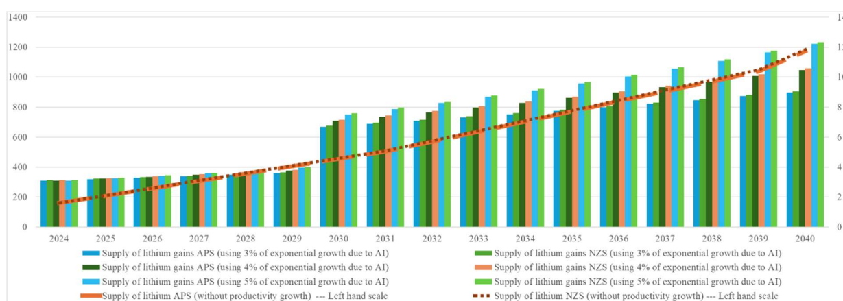
Fig. 7: Supply gains from productivity growth via AI investment and recycling for lithium. This figure illustrates projected lithium supply under the APS and NZS, incorporating different assumptions about annual production gains enabled by AI and recycling. The left-hand y-axis (measured in tonnes) represents the total supply, while the right-hand y-axis applies to the baseline APS and NZS supply trajectories without productivity growth, shown as dashed lines. Bar segments represent lithium supply projections with 3 per cent, 4 per cent and 5 per cent annual exponential productivity growth due to AI, applied to both APS (blue, dark green, and light blue bars) and NZS (brown, orange, and light green bars) trajectories, respectively. The dotted lines show lithium supply in the absence of any productivity gains, under both APS (red dashed) and NZS (brown dashed).
