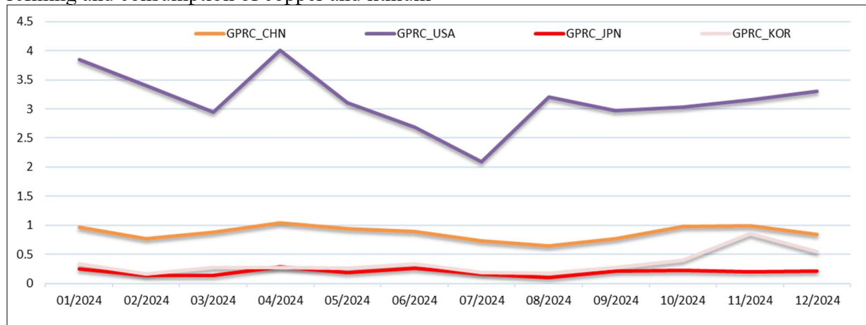
Supplementary Fig. 2 Geopolitical risk indicators for principal refining and consumption countries for copper and lithium. This figure displays the monthly geopolitical risk indicators for four major copper and lithium refining and consumption countries— China (GPRC_CHN), USA (GPRC_USA), Japan (GPRC_JPN), and South Korea (GPRC_KOR)—from January to December 2024.
